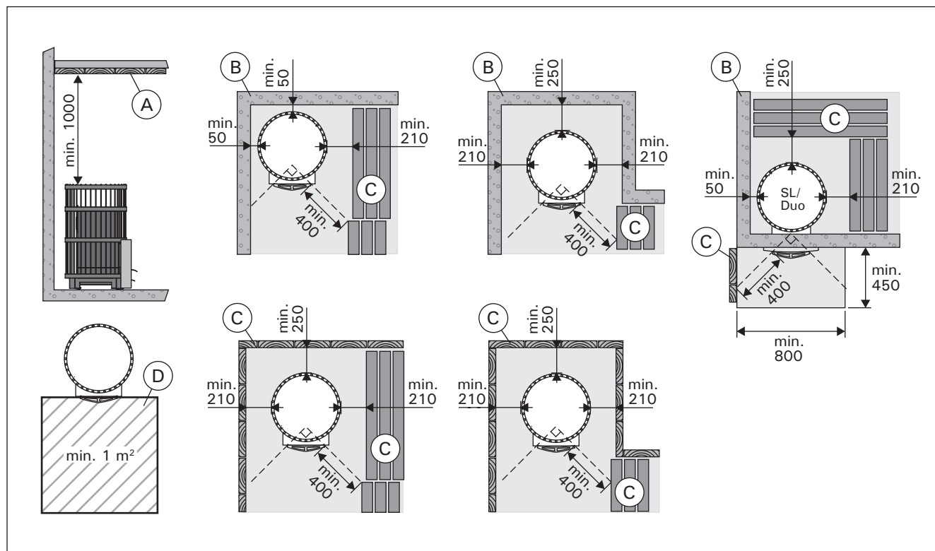
Figure 8. Safety distances (in millimeters)
