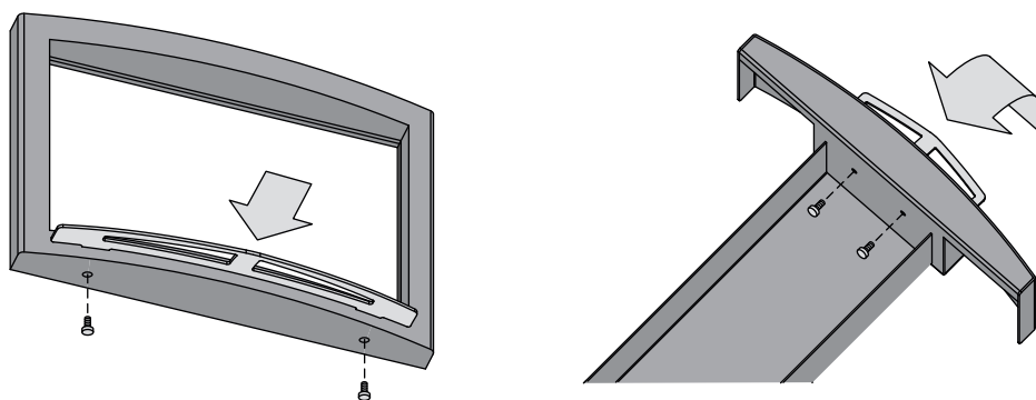
Figure 16. Installing the handles Obr. 16. Instalace madel
